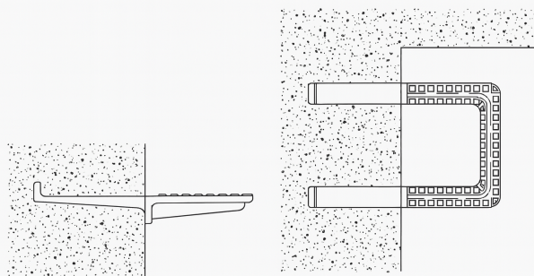
FIXING DETAILS IN CONCRETE
